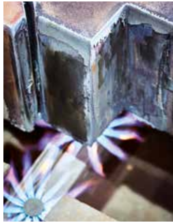
Pre-heating
